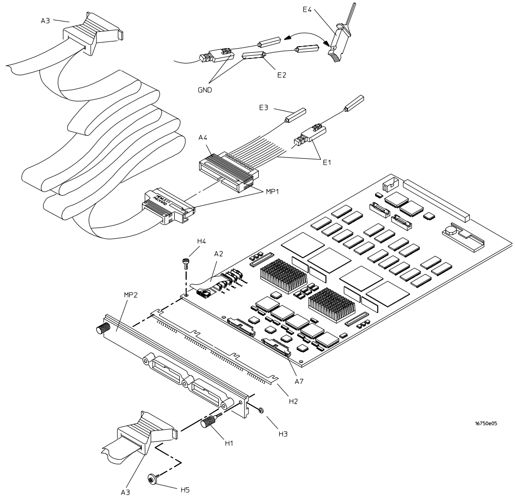
Exploded view of the 16750/51/52A logic analyzer
